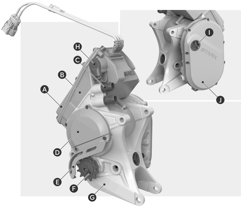
POWERTRAIN (MOTOR + INVERTER)
